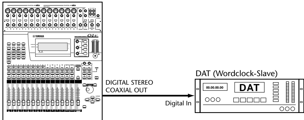
01V (Wordclock-Master)
