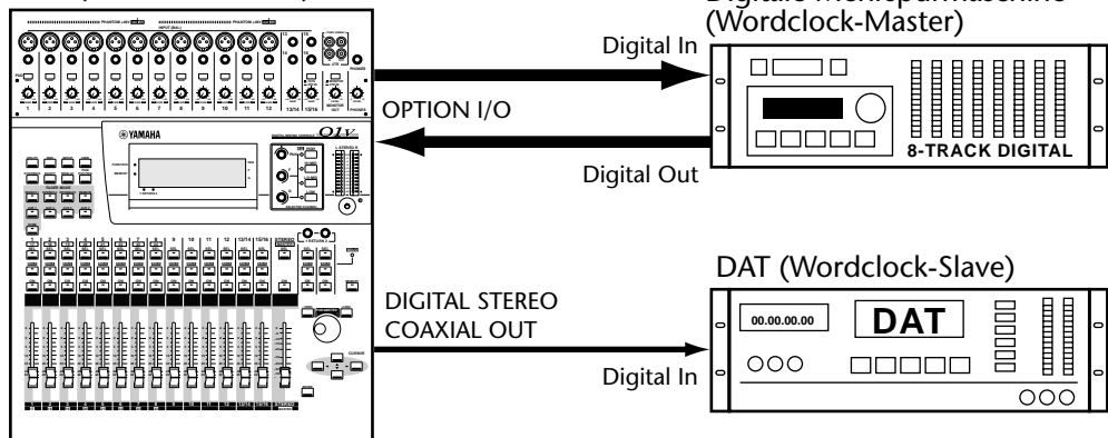
01V (Wordclock-Slave)
